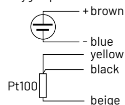
Oxygen probe with Pt100
